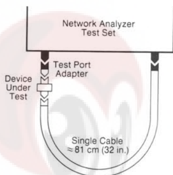
Configuration A For HP 8719A/8720B Network Analyzer or HP 8514B/8515A Test Sets (3.5 mm test port)
